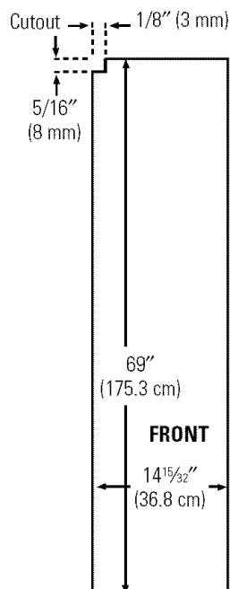
Freezer Panel Without Dispenser
