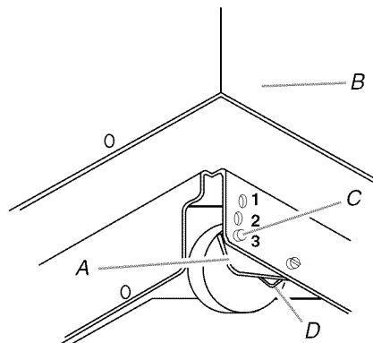
A. Wheel bracket assembly
