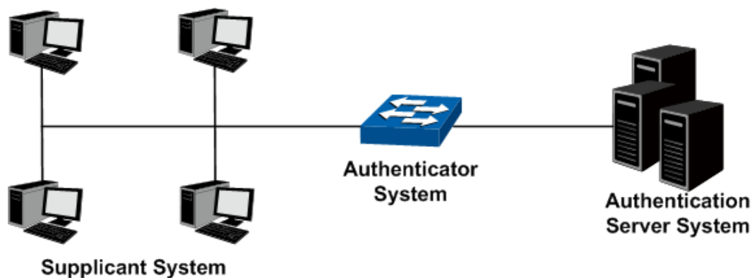
Figure 1-1 802.1x Topology
