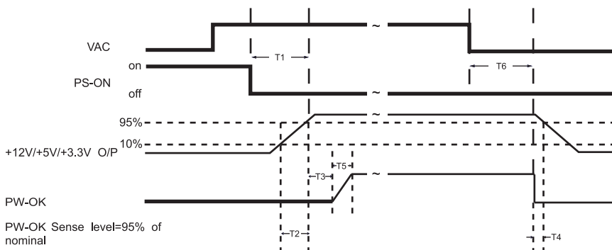
Figure 2. PS-OK Timing Sequence
