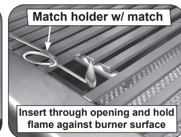
Fig. 37-3 Manual lighting via match holder
