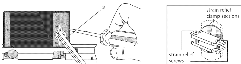
Fig.27 Inserting the power cord
