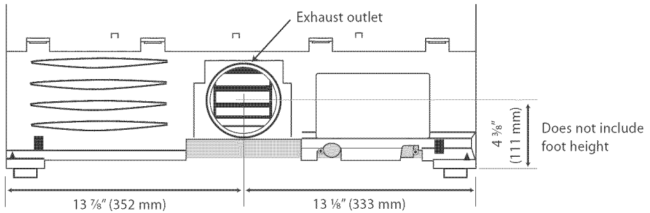
Fig.7 Exhaust outlet dimensions
