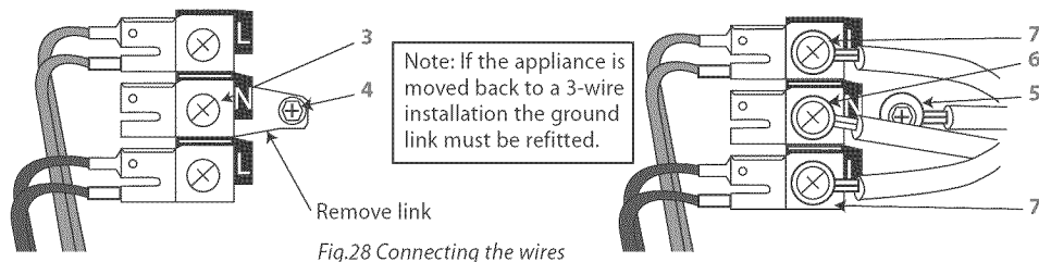
Fig.28 Connecting the wires
