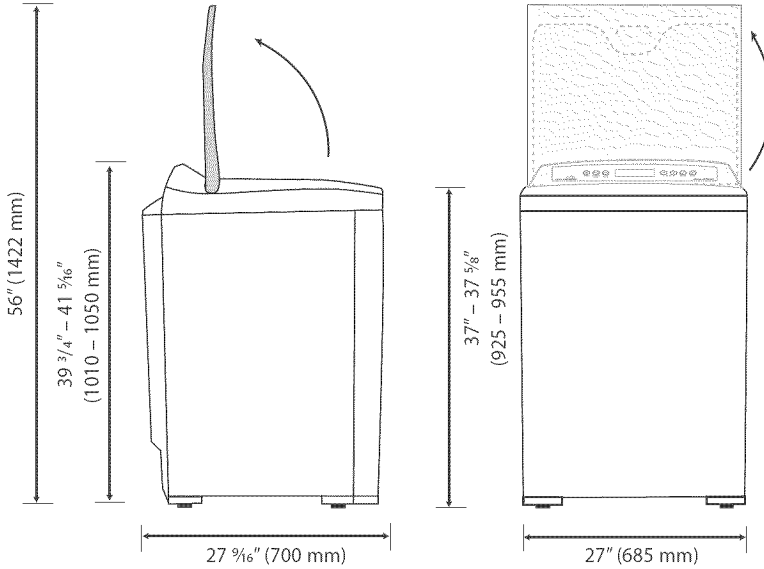
Fig.6 AeroSmart dimensions
