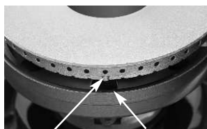
locator key burner base notch
