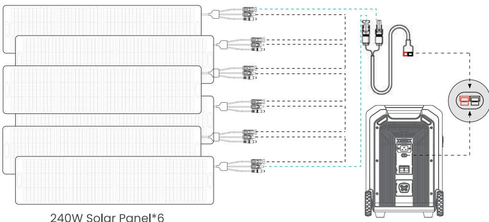
240W Solar Panel*6
