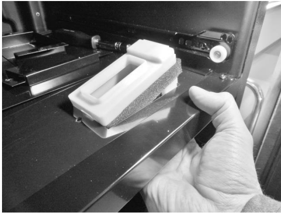
Rear Damper
