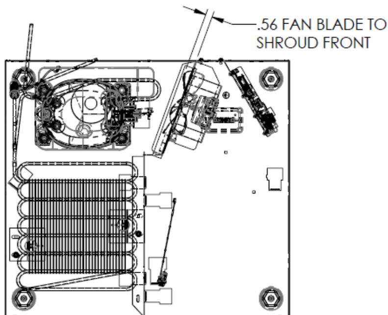
TOP VIEW SCALE 1 : 8
