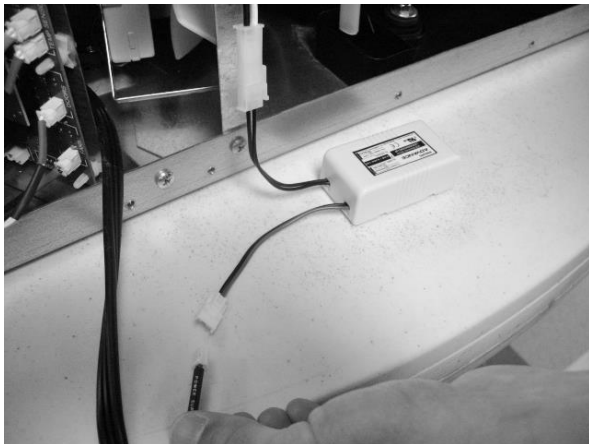
Connect the black and white wires from connector 3 (harness A) and the black and red wires from connector 4 (harness B) to the appropriate terminals on the power supply.
