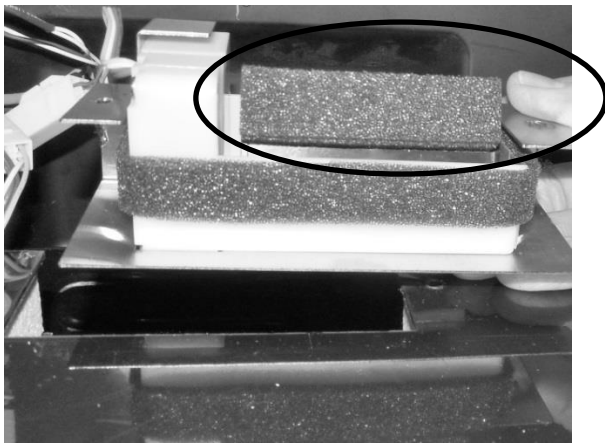
Front View: Rear damper in the open position: NOTE the insulation on the back of the damper door.
