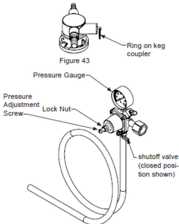
Figure 44 (Regulator for Single Dispense Tower)
