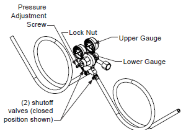
Figure 45 (Regulator for Double Dispense Tower)
