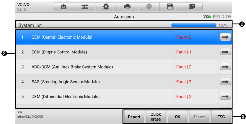
Figure 4-12 Auto Scan Screen
