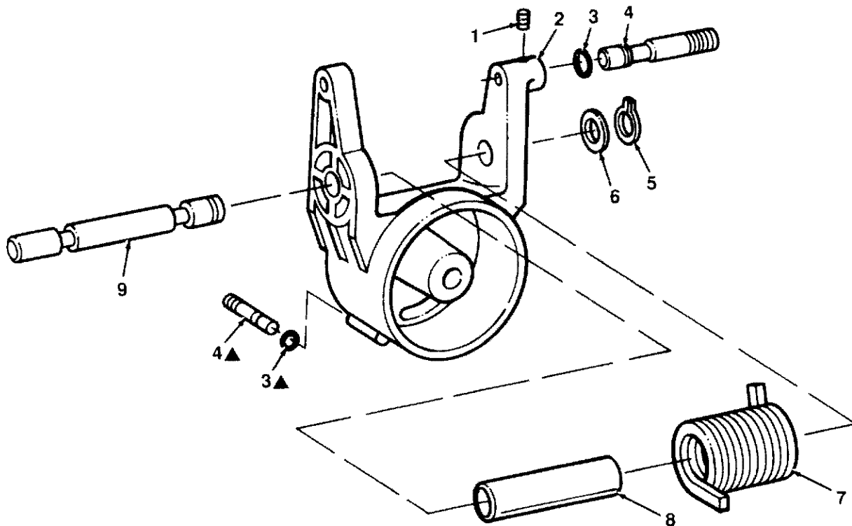
FIGURE 3—PIVOT ASSEMBLY
