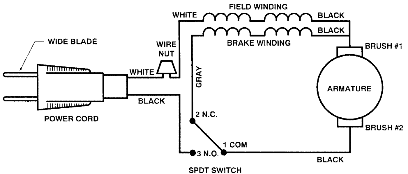
Circuit Diagram
