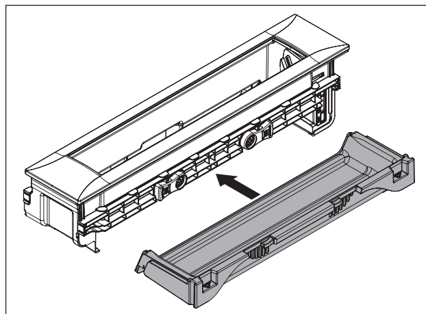
Fig. 8.5 Installing the maintenance tray
