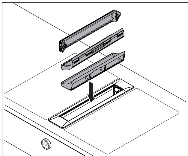
Fig. 8.2 Fitting the components
