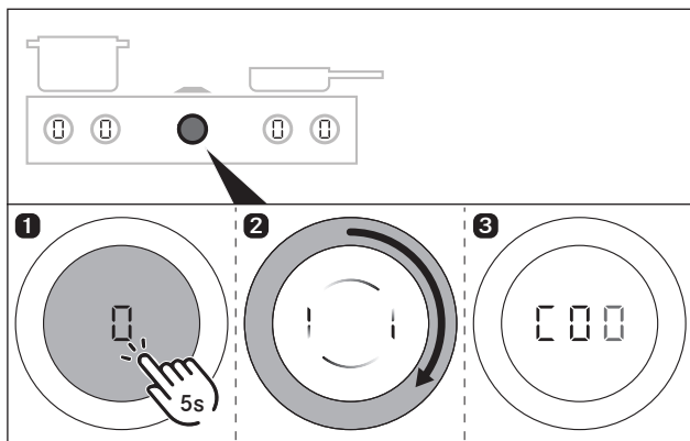
Fig. 7.39 Calling up the menu
