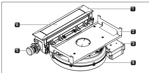
Fig. 4.6 Cooktop extractor system PKAS3/PKAS3AB
