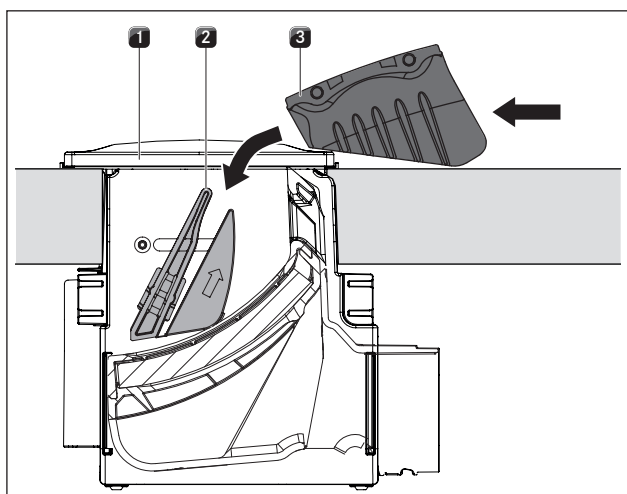
Fig. 8.3 Fitting the cover flap
