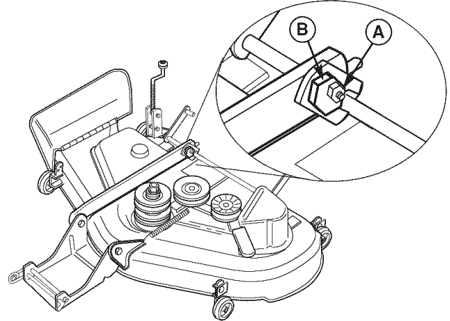
Figure 40. Front-to-Back Leveling
