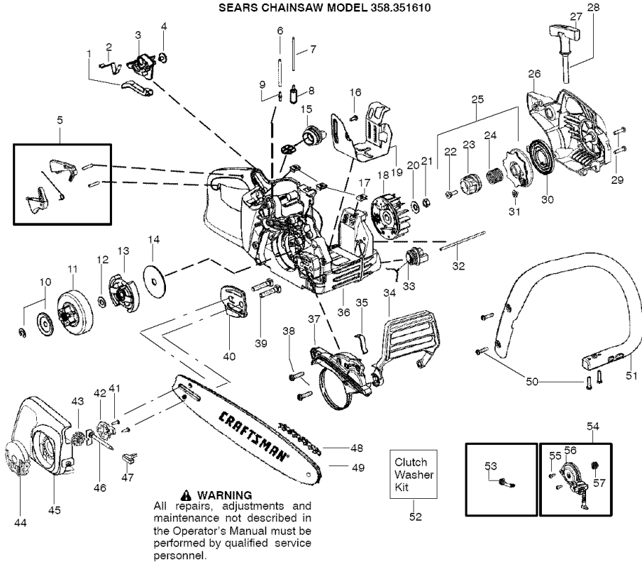
SEARS CHAINSAW MODEL 358.351610
