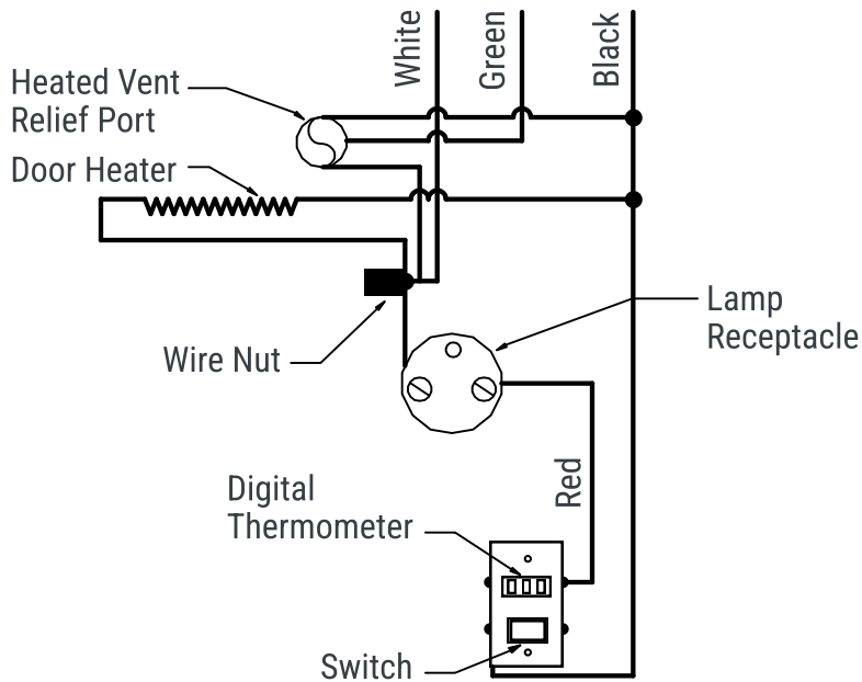
WIRING DIAGRAM
