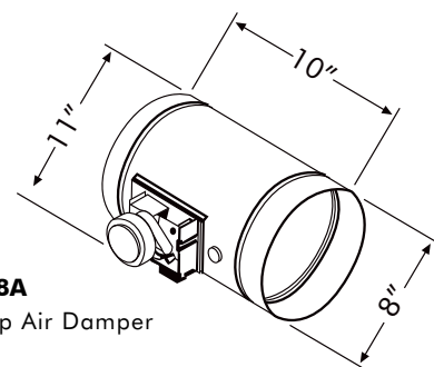
MUA006A Make-Up Air Damper
