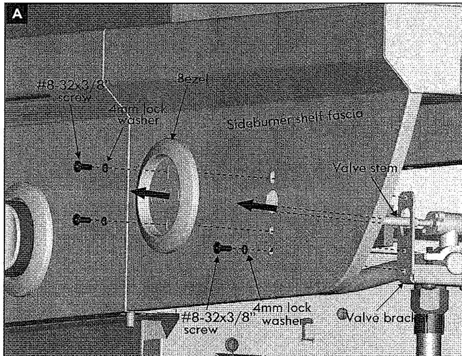
#8-32x3/8" screw Qty.3
