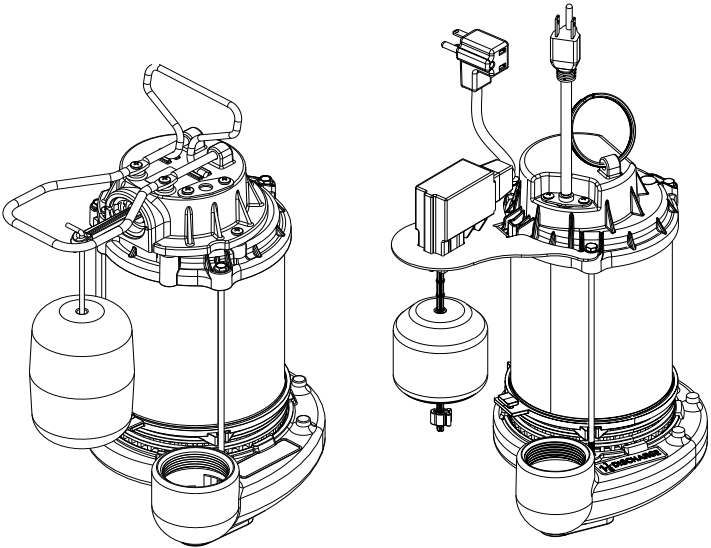
Vertical Float Switch
