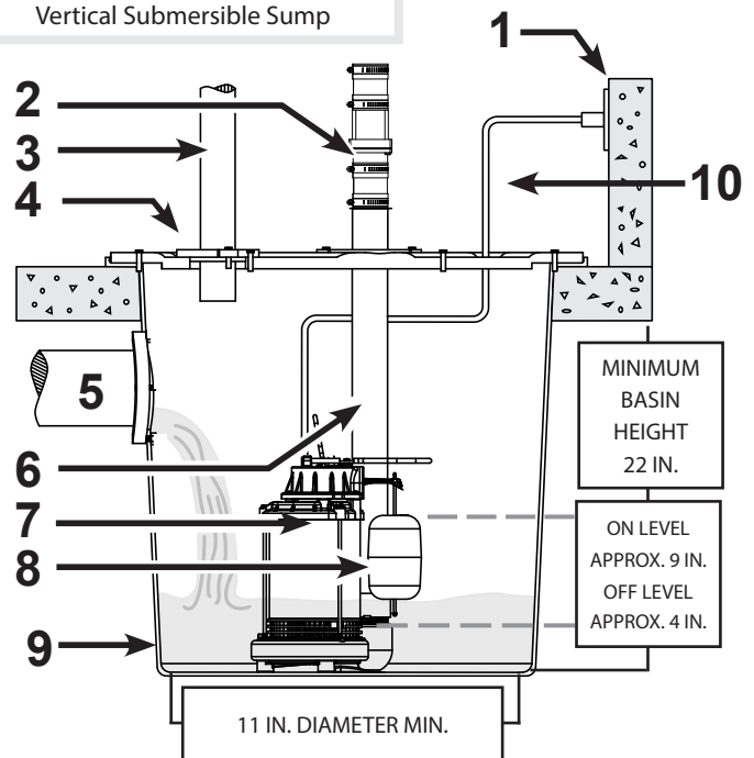
Vertical Submersible Sump
