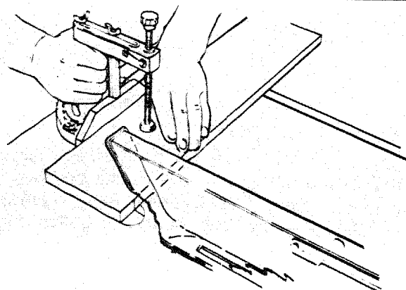
BLADE GUARD SHOWN IN "PHANTOM" FOR PICTURE CLARITY
