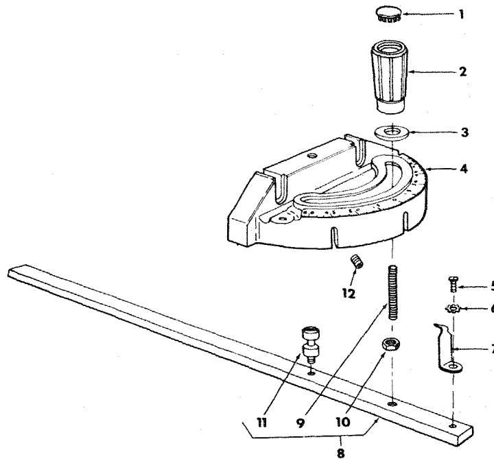
FIGURE 8 - MITER GAUGE ASSEMBLY
