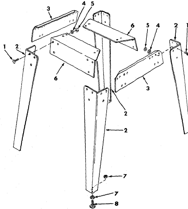
FIGURE 7 - LEG SET
