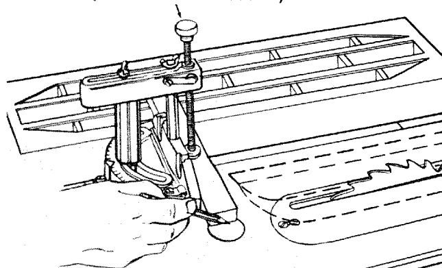
SHOWN WITH HOLD-DOWN CLAMP (OPTIONAL ACCESSORY)
