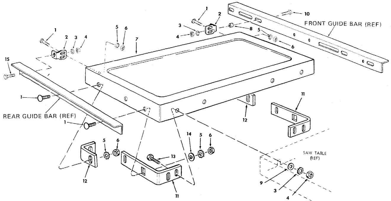
FIGURE 6 - TABLE EXTENSIONS
