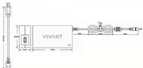
Power adapter and charging cable
