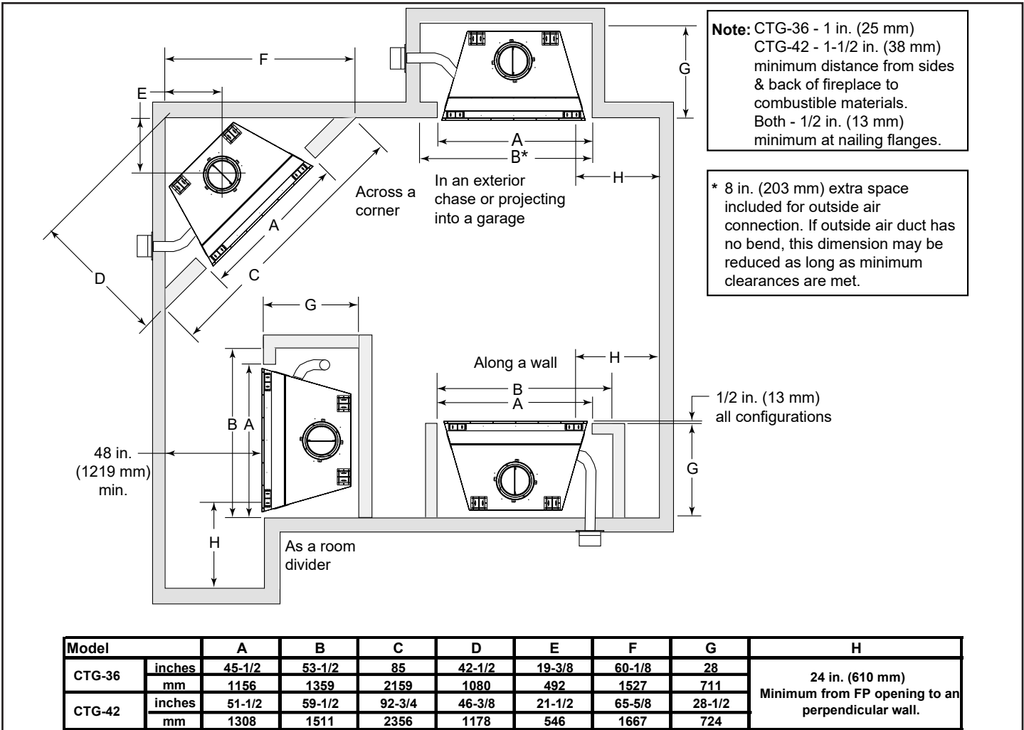
Figure 2.2 Fireplace Locations
