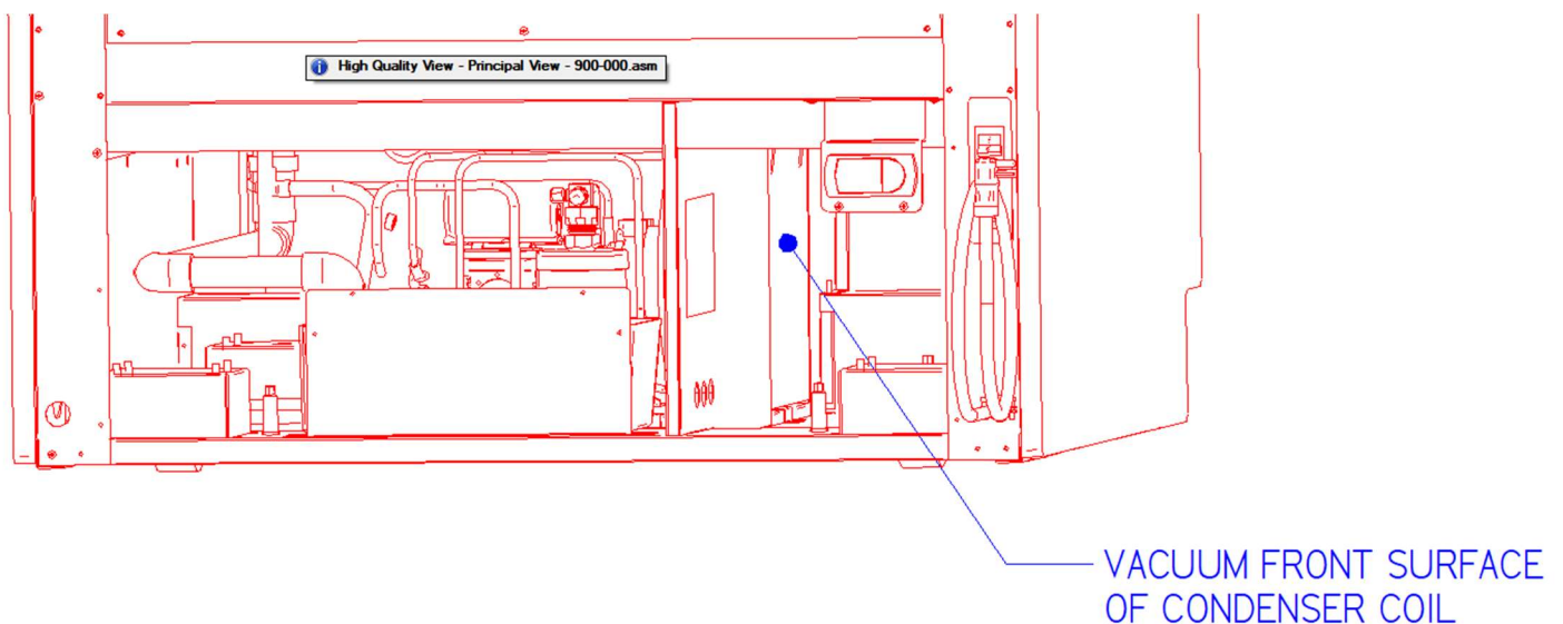
Figure 1 - Condenser Cleaning
