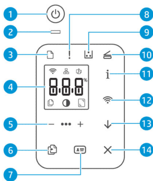
Control panel view (sdn/sdw model)
