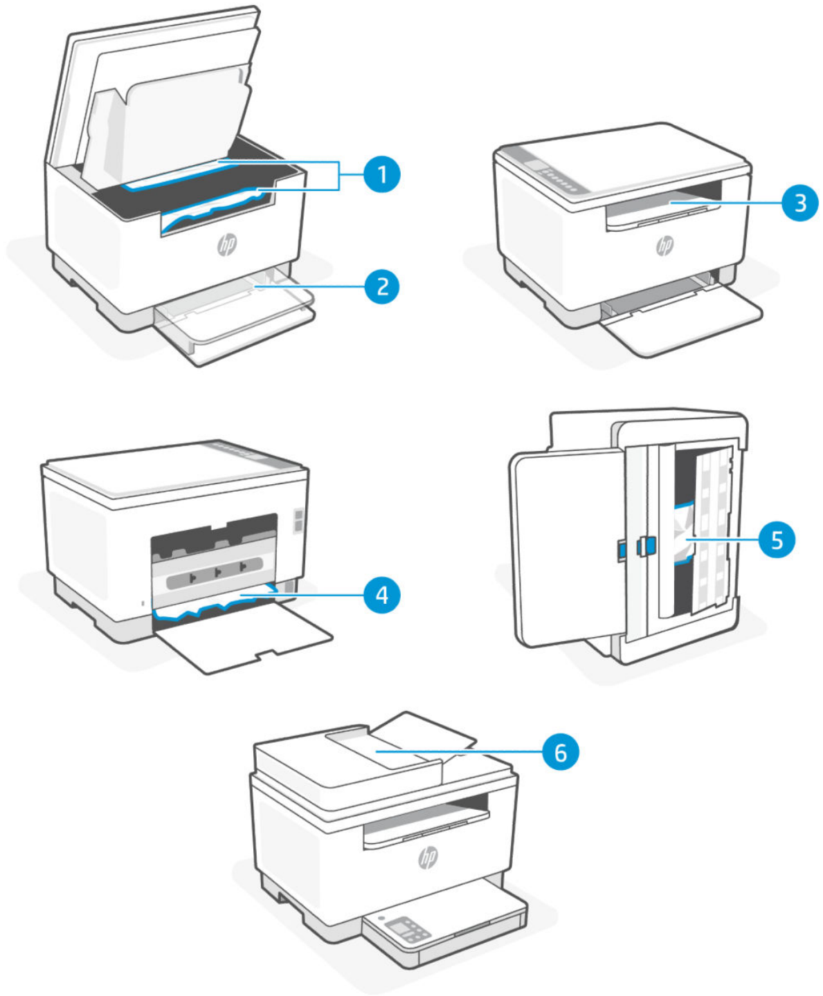
Jam locations (d/dw and sdn/sdw models)
