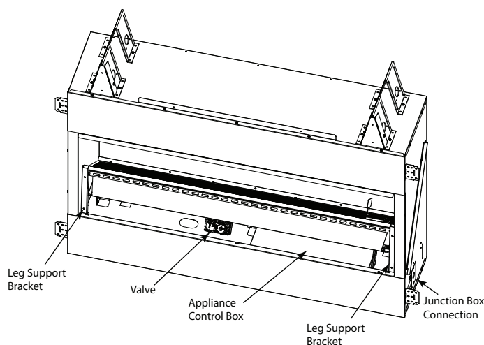
Figure 6.1. Appliance With Engine Lifted
