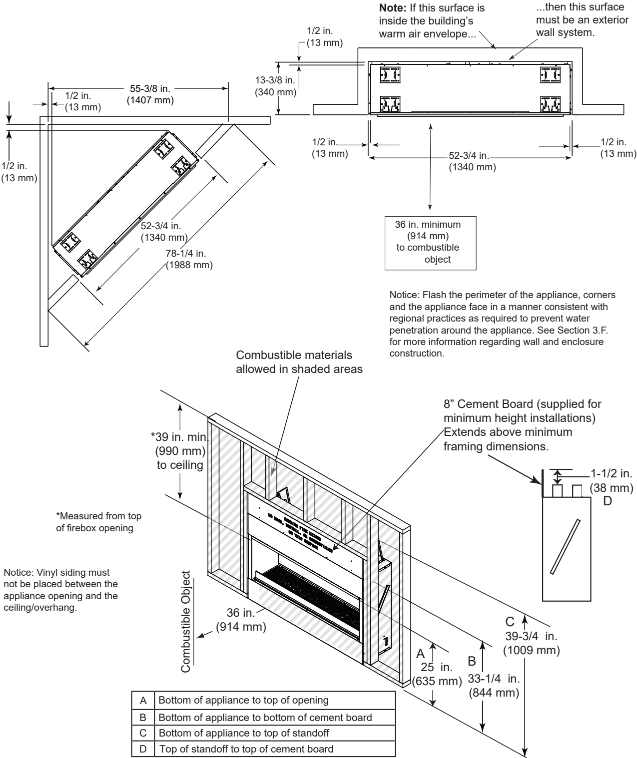
Figure 3.2. Appliance Locations and Framing Dimensions - ODLANAIG-48
