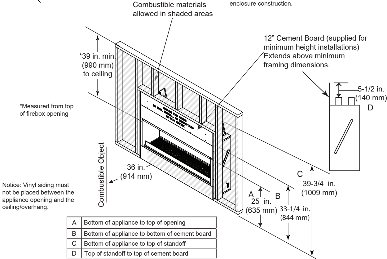
Figure 3.3. Appliance Locations and Framing Dimensions - ODLANAIG-60 10 Outdoor Lifestyles by Hearth & Home Technologies • Lanai 48/60 Installation Manual • 4111-901 Rev. I • 06/23
