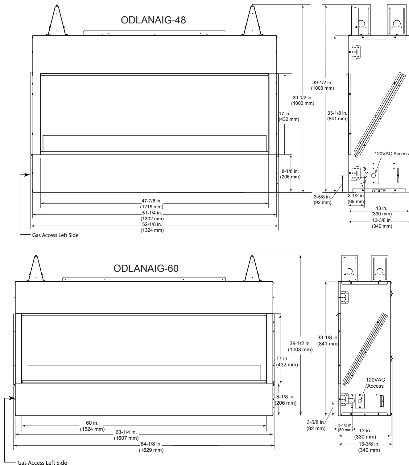
Figure 3.1. Appliance Dimensions – ODLANAIG-48/60 Outdoor Lifestyles by Hearth & Home Technologies • Lanai 48/60 Installation Manual • 4111-901 Rev. I • 06/23
