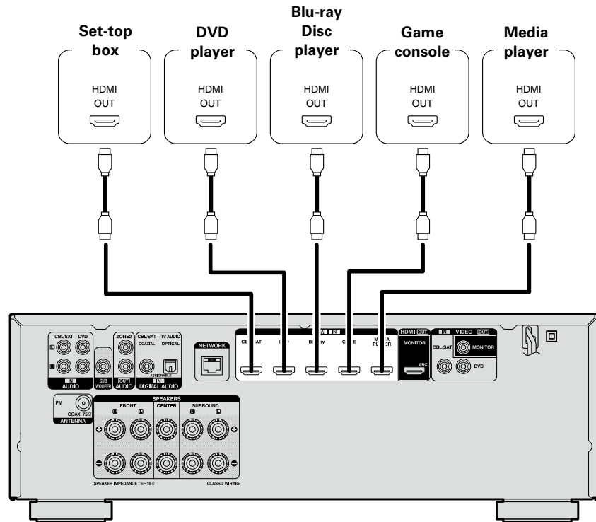
[Rear panel]
