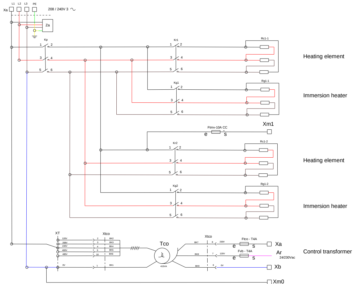
Power diagram 6GN2/1 and 10GN1/1 – 208V- 240V
