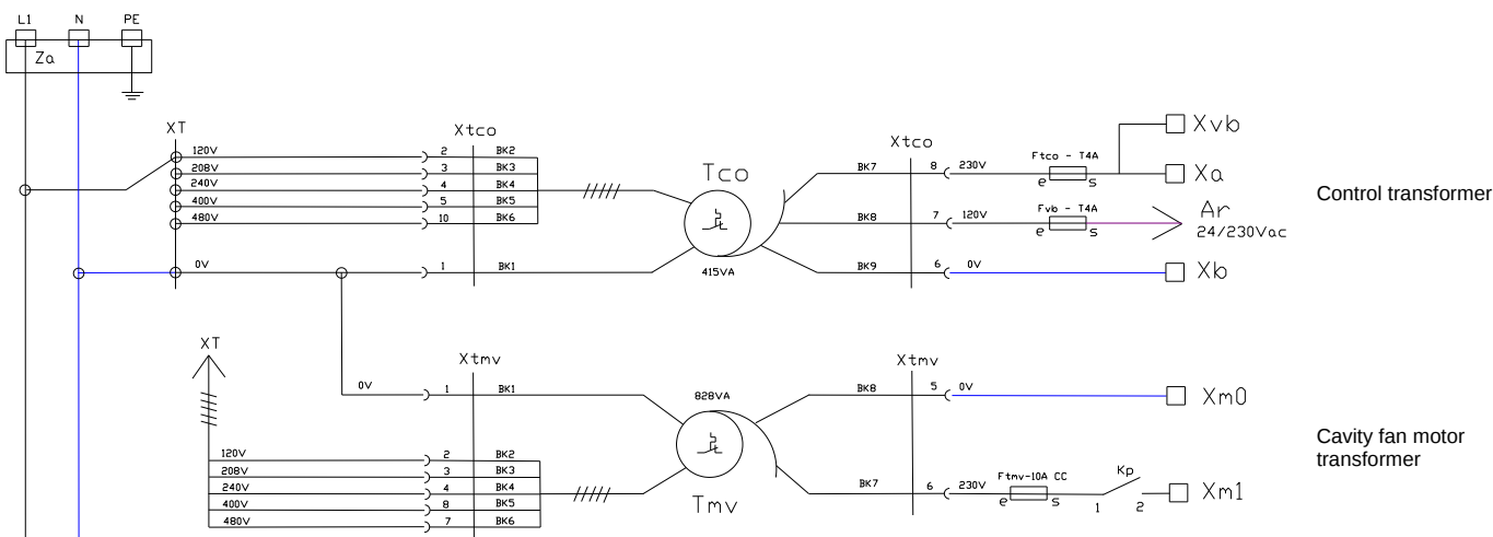
Power diagram 6 & 10 GN 2/1
