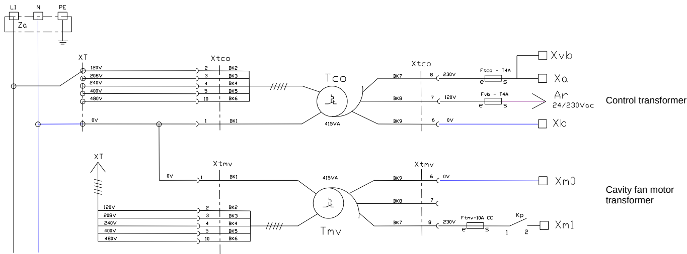
Power diagram 6 & 10 GN 2/1
