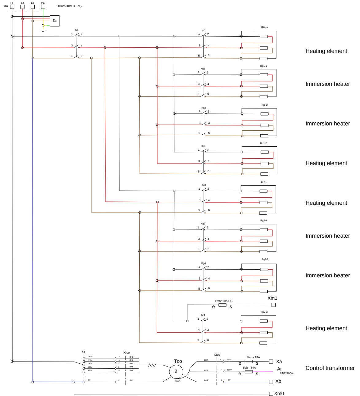
Power diagram 10GN2/1 – 208V- 240V
