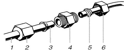
1. Line to refrigerator 2. Nut (provided) 3. Bulb 4. Coupling (provided) 5. Ferrule (purchased) 6. Nut (purchased)
