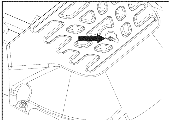
Deck spindle
