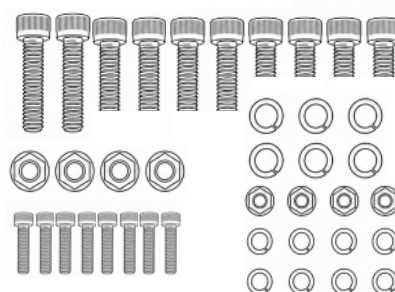
M8 × 30 mm Screws × 2 M8 × 25 mm Screws × 4 M8 × 12 mm Screws × 4 M8 Nuts × 4 M8 Spring Washers × 6 M5 Screws × 8 M5 Nuts × 4 M5 Spring Washers × 8
