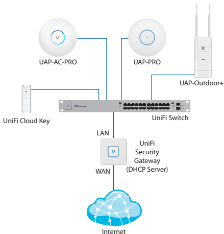
Sample Network Diagram
