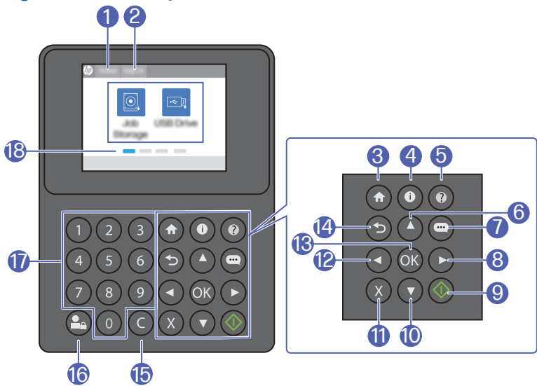
Figure 1-8 Control-panel view
