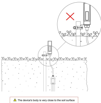
Figure 30 The device's body is very close to the soil surface
