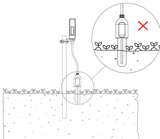
Figure 29: The sensor probe should be inserted totally inside the soil
