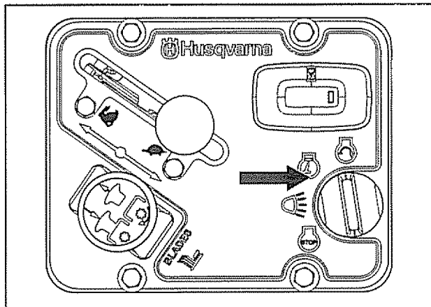
Ignition switch
