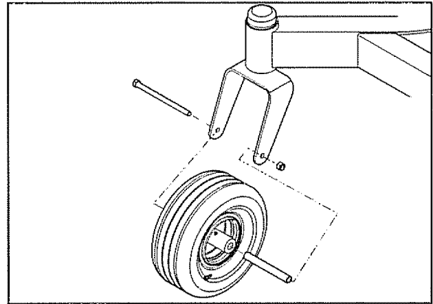
Caster wheel
