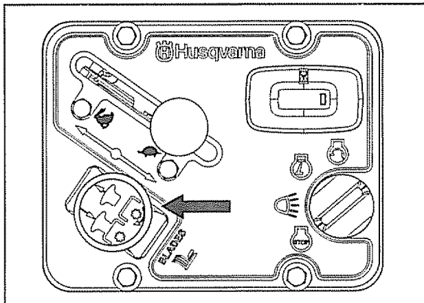
Blade switch
