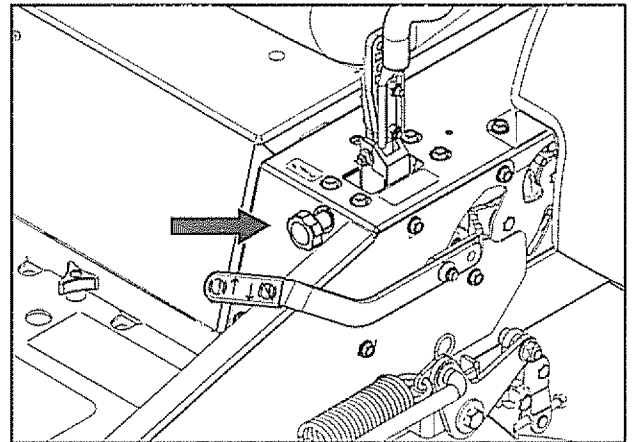
Tracking adjustment
