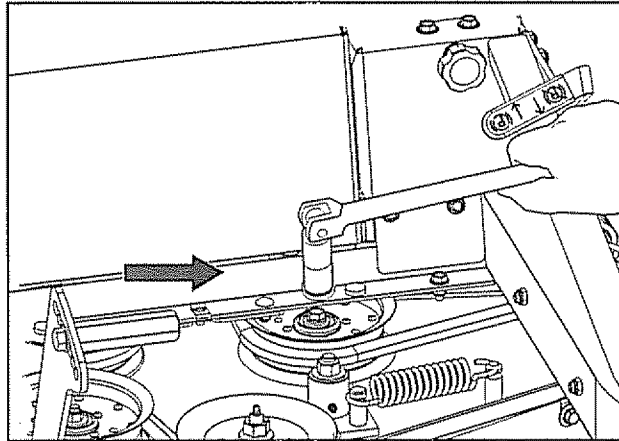
Slackening the belt tensioner
