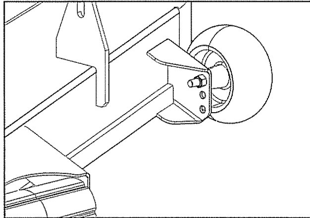
Anti-scalp rollers
