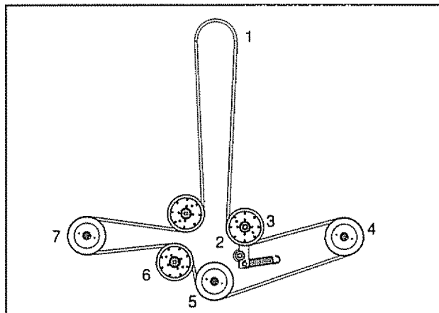
Belt routing, deck belt
