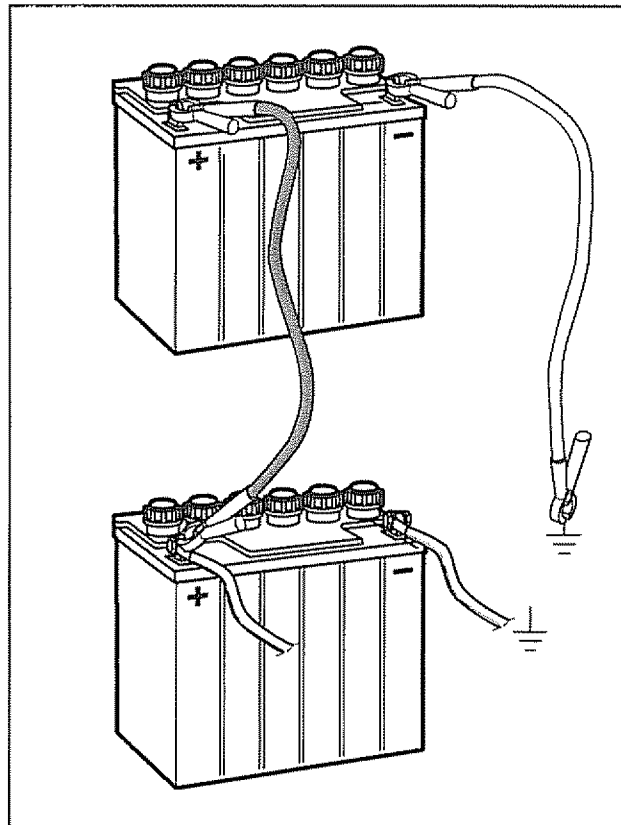
Jumper cable connection
