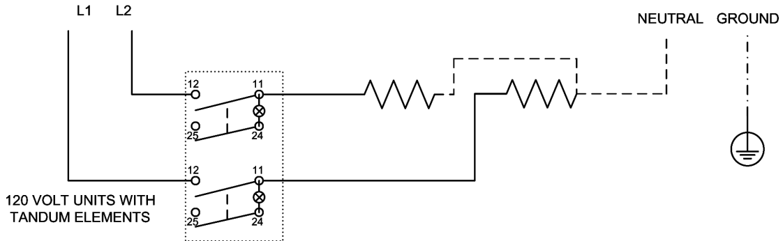
REMOTE SWITCH WITH INDICATOR LAMPS
