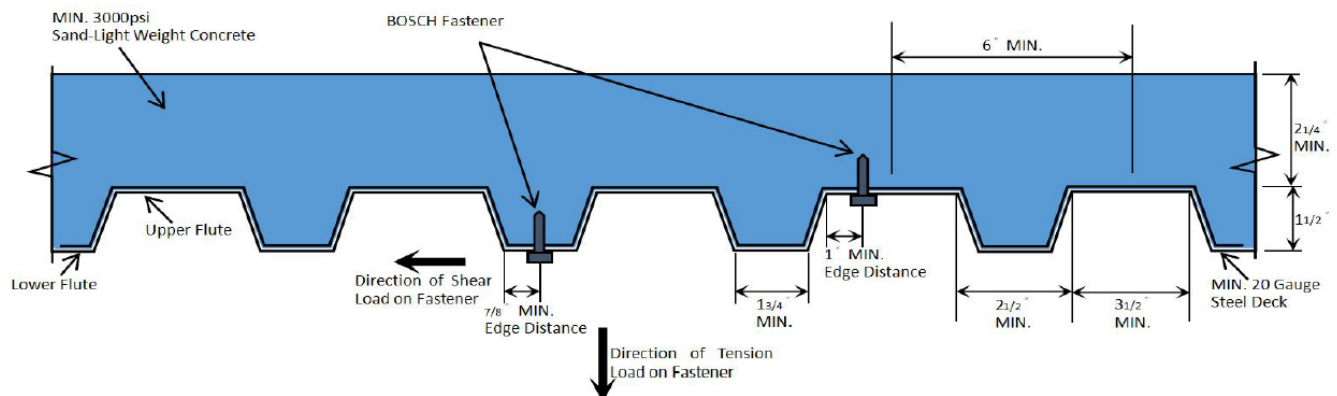
FIGURE 6—BOSCH FASTENER LOCATIONS IN 1½-INCH-DEEP B-DECK PANEL
