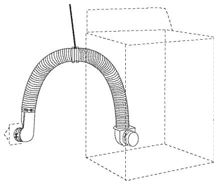
Vent system installed over-the-top with one offset and one standard elbow
