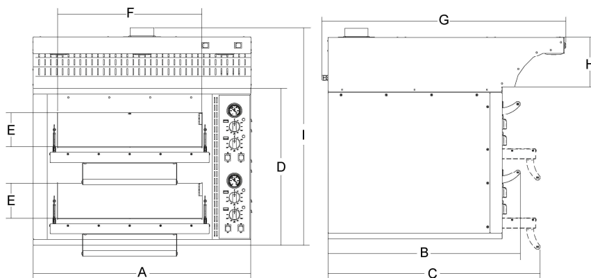
FIG. n°2 - Overall dimensions
