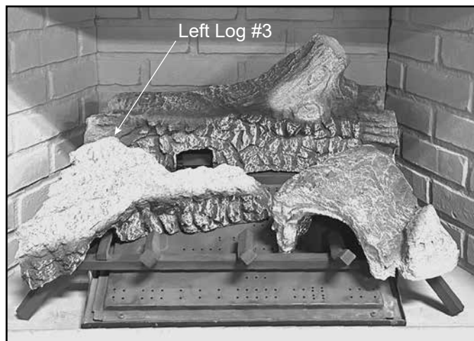
Figure 4 Left Log #3
