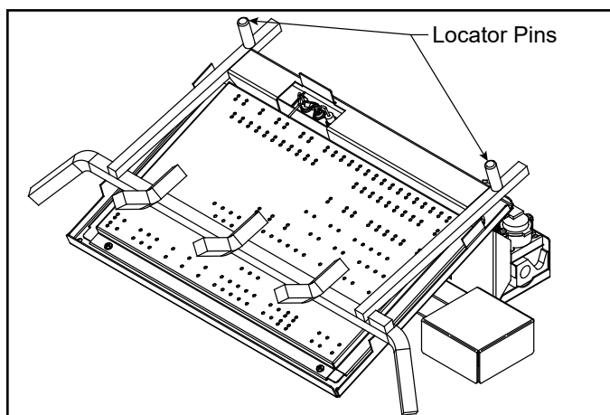
Figure 1 Locator Pins
