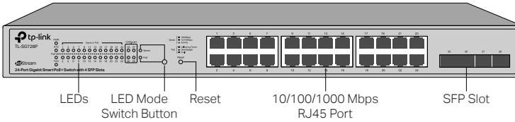
Figure 1-6 Front Panel of TL-SG728P
