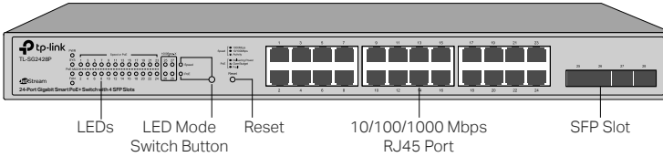
Figure 1-4 Front Panel of TL-SG2428P
