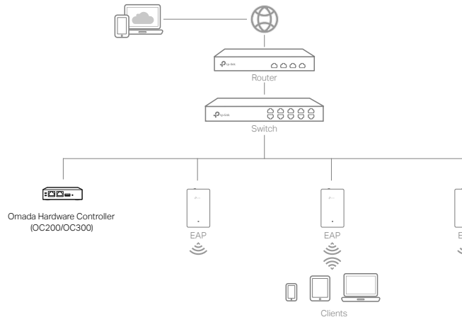
Figure 4-2 Manage the network via Omada Hardware Controller
