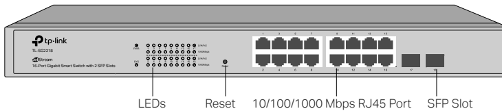
Figure 1-1 Front Panel of TL-SG2218
