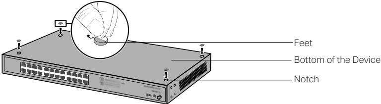
Figure 2-1 Desktop Installation
