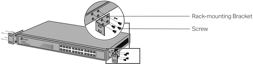
Figure 2-2 Bracket Installation
