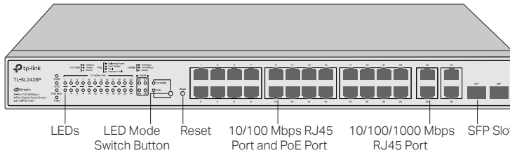
Figure 1-5 Front Panel of TL-SL2428P
