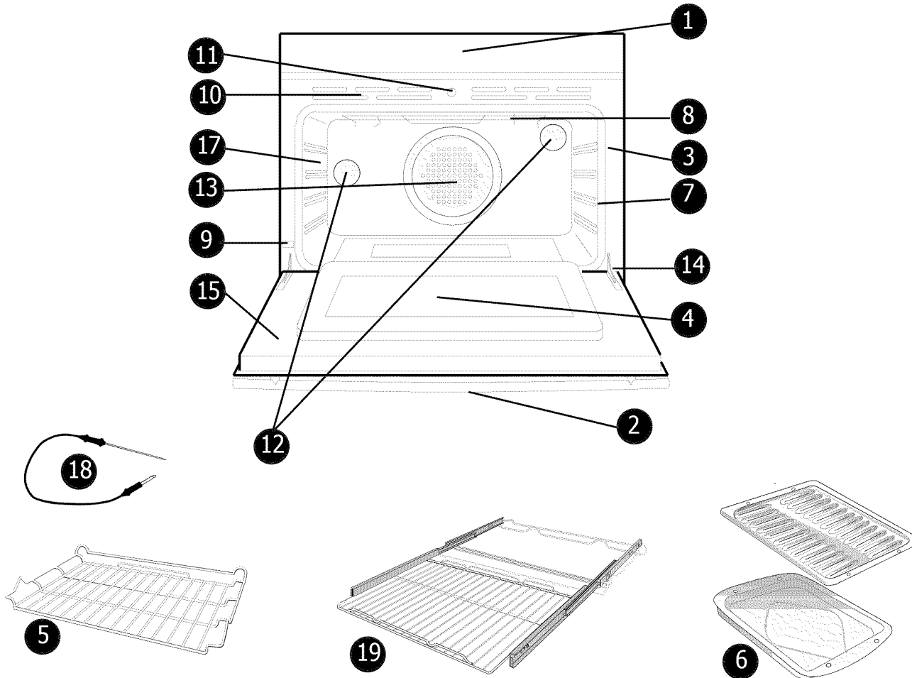
Figure 1: Oven Parts
