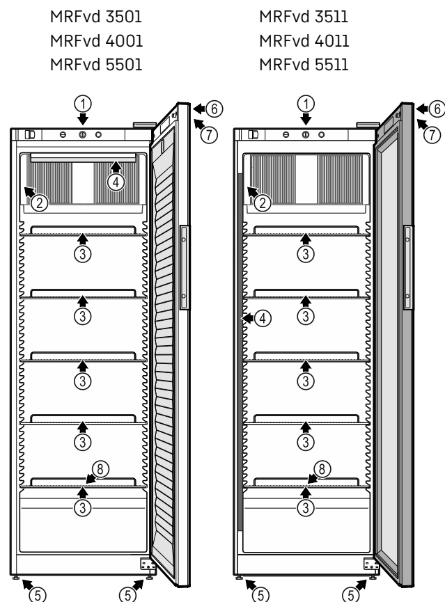
Fig. 1 Basic equipment
