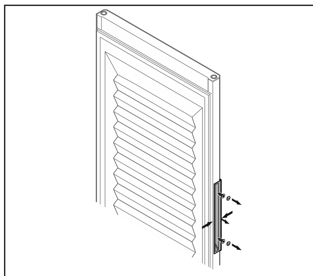
Fig. 18 Insulated door*
