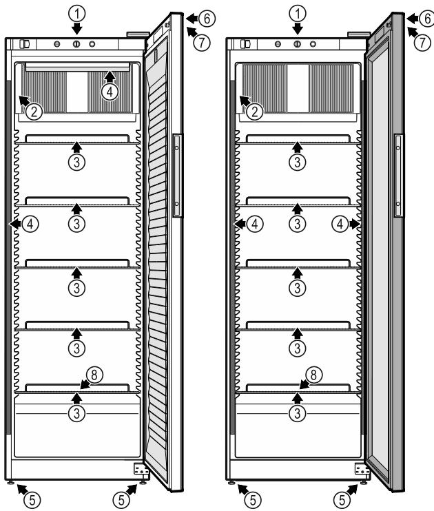
Fig. 2 Variants
