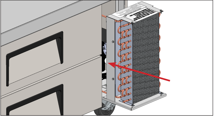
Fig. 6. Carefully slide the condensing unit back into position and reinstall the bolts.
