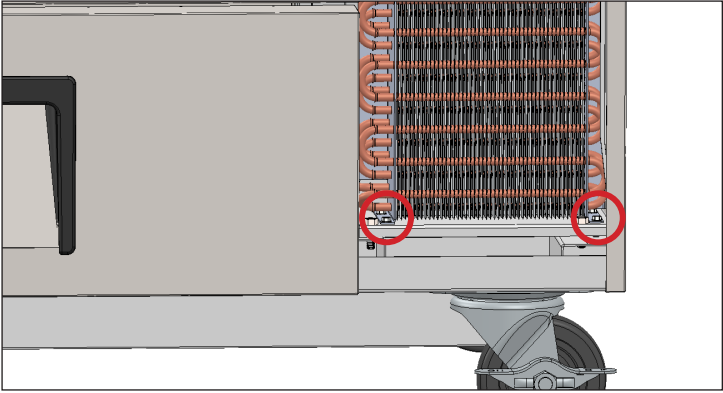
Fig. 4. Condenser base bolt locations.
