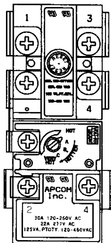
UPPER THERMOSTAT ADJUSTABLE BEHIND UPPER ACCESS PANEL
