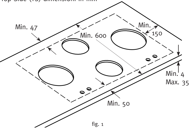
Top Side (TS) dimensioni in mm
