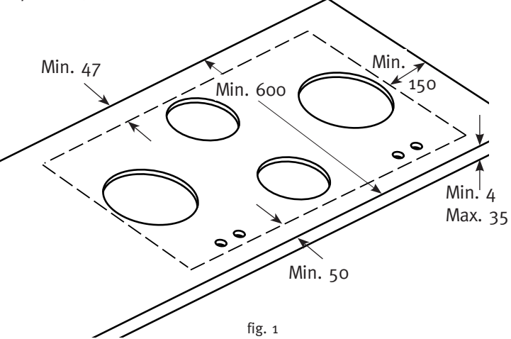
Top Side (TS) maten in mm
