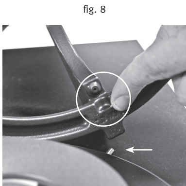
Pan support with centering cams
