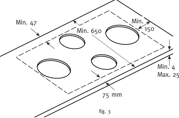
Front Side (FS) maten in mm
