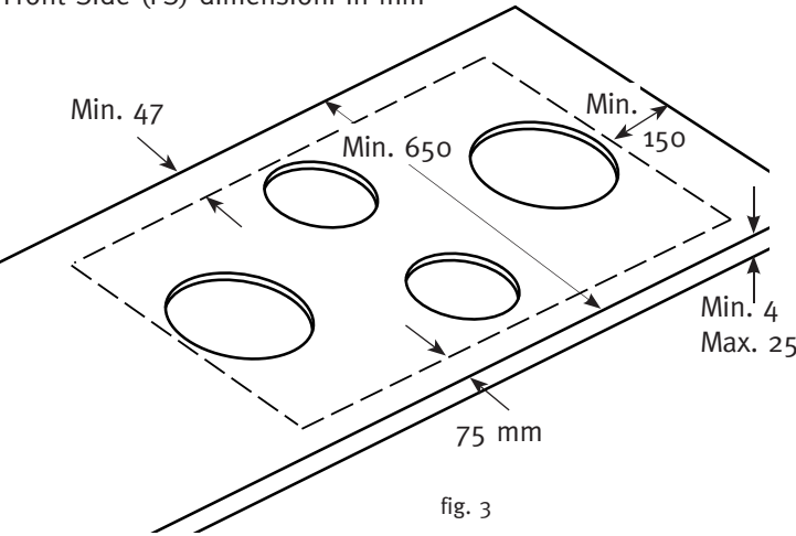
Front Side (FS) dimensioni in mm
