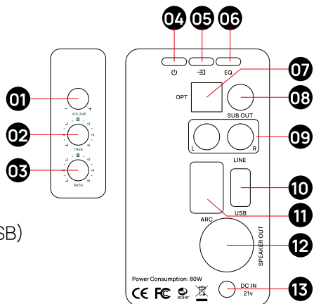
Active Speaker
