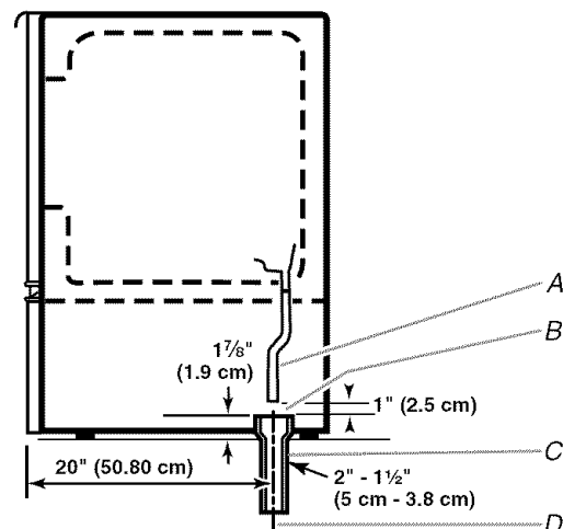
A. Drain hose B. 1" (2.54 cm) air gap C. PVC drain reducer D. Center of drain should be 20" (50.80 cm) from front of door, with or without the 3/4" (1.91 cm) panel on the door. The drain should also be centered from left to right (8 1/16" from either side of the ice maker).
