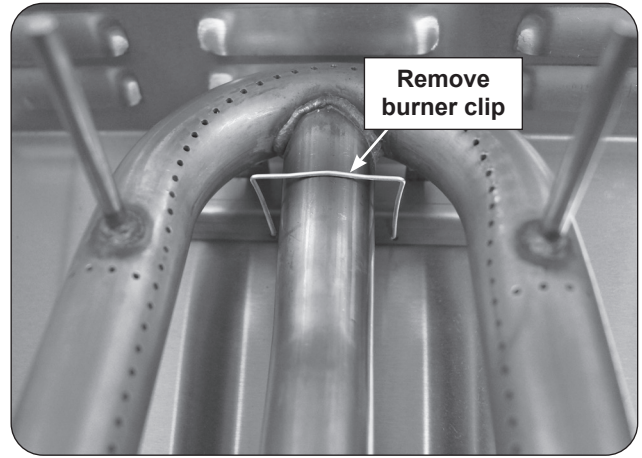
Fig. 38-1 Main burner removal
