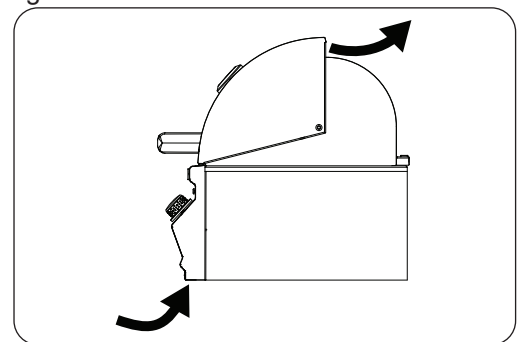
Fig. 31-1 Airflow diagram
