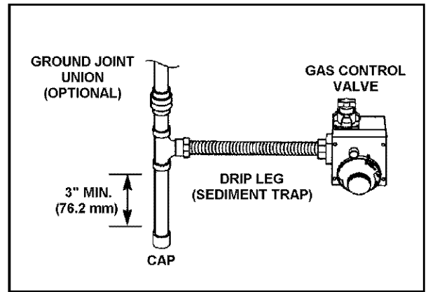
FIGURE 19. GAS PIPING WITH FLEXIBLE CONNECTOR.
