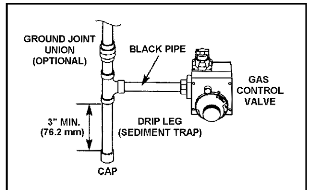
FIGURE 20. GAS PIPING WITH ALL BLACK IRON PIPE TO GAS CONTROL.
