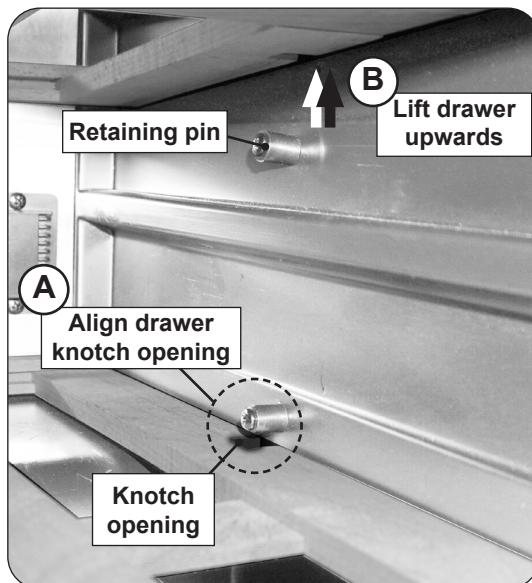
Fig. 10-3 Lower zone wooden shelf removal
