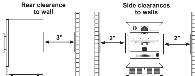
Fig. 4-2 Cut out wall clearances
