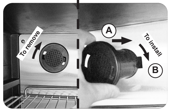
Fig. 11-1 Charcoal filter
