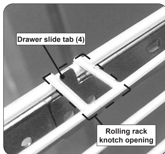
Fig. 10-2 Top rolling rack detail
