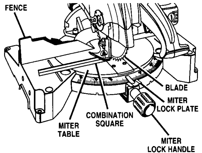
CORRECT VIEW OF BLADE SQUARE WITH MITER TABLE
